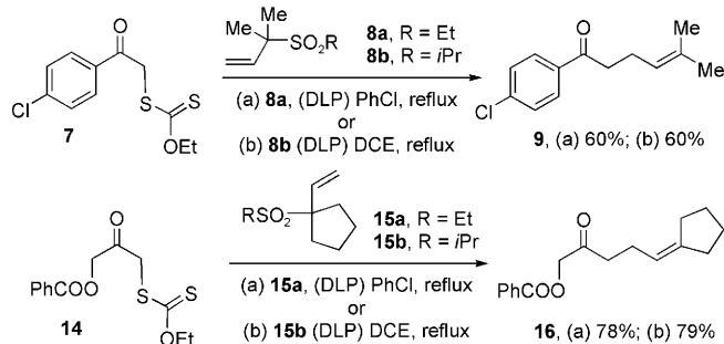
Scheme 3. Resolutions of premature allyl sulfone isomerization. DLP = dilauroyl peroxide.
